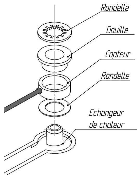
Fig.8 – Capteur de surchauffe (thermocouple)
