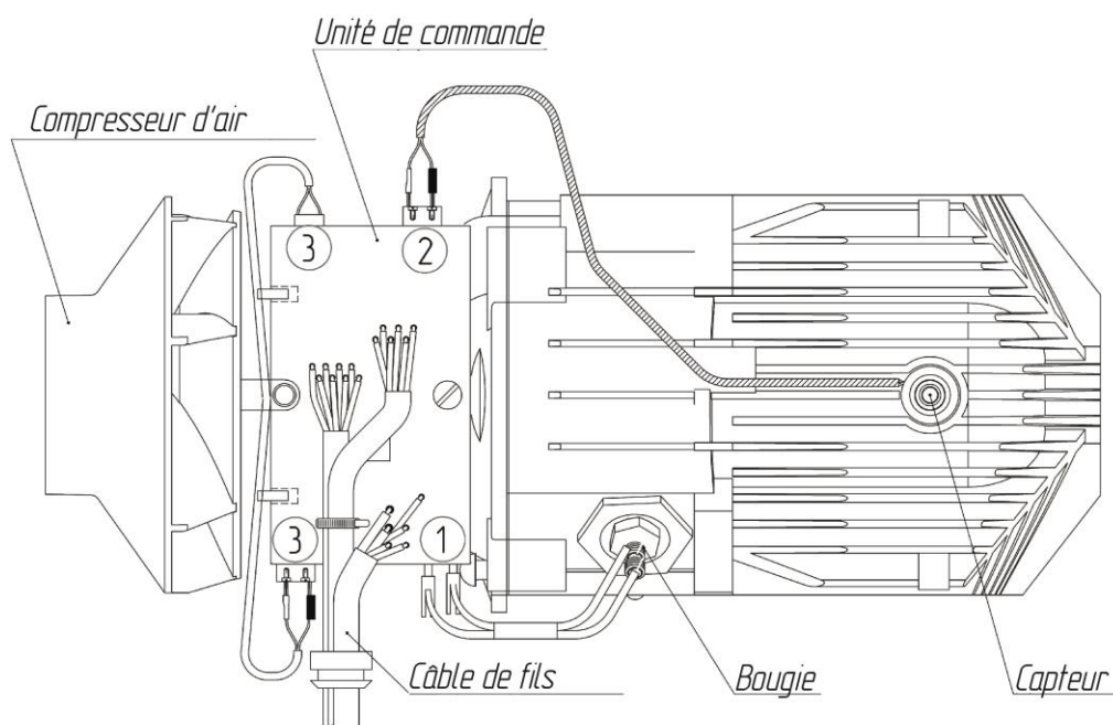
Figure 2 - Élément chauffant
